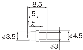
PB107形
