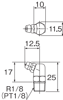
B-PT1/8形
