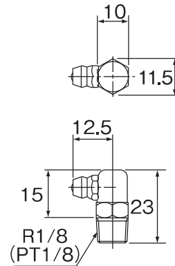
C-PT1/8形
