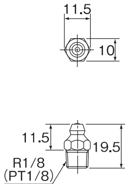
A-PT1/8形
